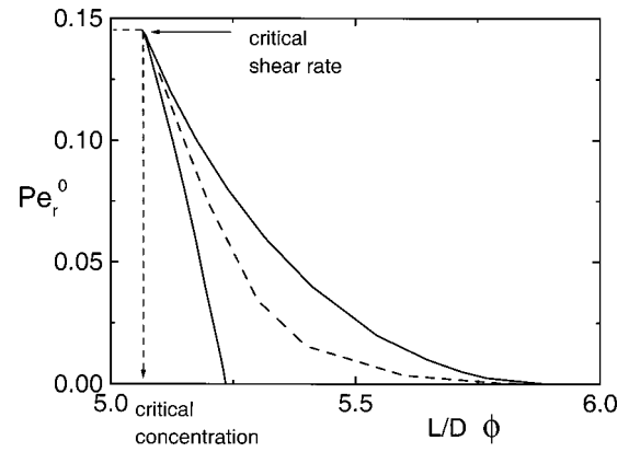
FIG. 3. Nonequilibrium spinodals. The lower solid line is the spinodal where the nematic phase becomes unstable on lowering the concentration (the nematic-to-paranematic spinodal), while the upper solid line is the spinodal where the paranematic phase becomes unstable on increasing the concentration (the paranematic-to-nematic spinodal). The dotted line is the predicted experimental curve as obtained from birefringence hysteresis experiments, as calculated from the equation of motion Eq. (16) (see Sec. II F).
