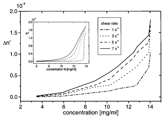
FIG. 8. Birefringence as a function of concentration for four shear-rates, which are indicated in the figure. The inset shows the theoretical prediction according to Eq. (16).
