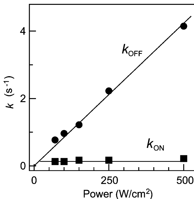
FIG. 5. Intensity dependence of the blinking rate constants of TMR-6-Cy5 molecules excited with the red laser. Each data point in this plot was obtained from the distribution of over 500 single molecules as explained in Fig. 4. The off rate is linearly dependent on the 640 nm excitation power, whereas the on rate is power independent.
