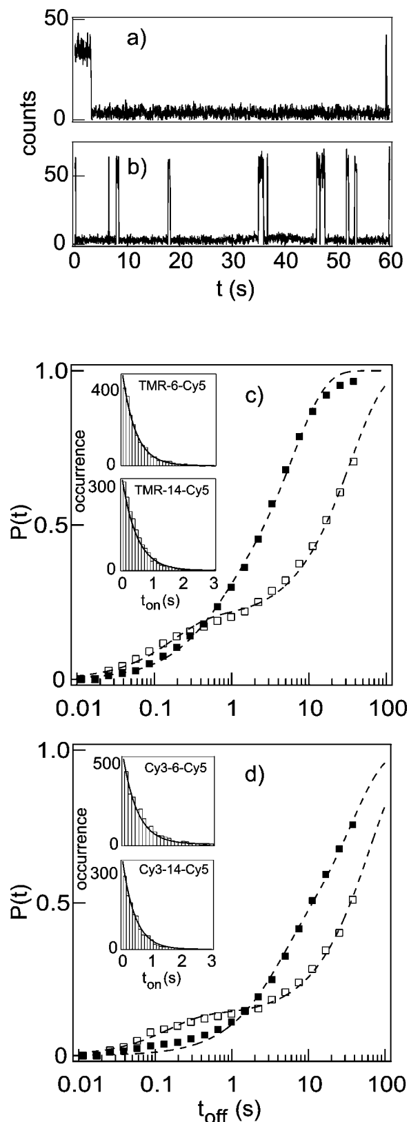
FIG. 6. Influence of donor proximity on the blinking times of Cy5 using 640 nm excitation ( 0.25 \text{kW}/\text{cm}^2 ). Typical time trace of the acceptor channel for (a) TMR-14-Cy5 and for (b) TMR-6-Cy5. The cumulative probability distribution P(t) is used to determine the characteristic dwell times of the Cy5 dark states for the TMR/Cy5 constructs (c) and the Cy3/Cy5 constructs (d). The dotted lines are double-exponential fits to P(t) for Donor-6-Cy5 (filled symbols) and Donor-14-Cy5 (open symbols); the average time scales and amplitudes are given in the text. The insets are distributions of the Cy5 on times yielding k_{\text{off}}\approx 2 \text{s}^{-1} in all cases.
