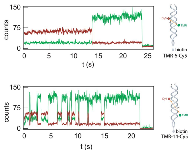
FIG. 1. Representative time traces of individual DNA molecules internally labeled with TMR and Cy5 fluorophores with an interdyde separation of six nucleotides (top panel) and 14 nucleotides (bottom panel). Schematics of the constructs are given to the right of the traces. The red lines correspond to counts (per 10 ms) from the acceptor channel and the green lines from the donor channel, excited by a 514 nm laser (0.5 kW/cm 2 at sample).
