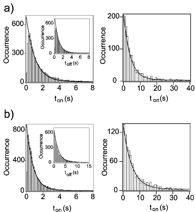
FIG. 2. a) Distributions of the low (off) and high (on) FRET dwell times obtained from single-molecule traces. The left panel corresponds to TMR-14-Cy5 and the right panel to TMR-6-Cy5. The main figures are for the distributions of t_{on} and the inset shows distributions of t_{off} . The solid lines are monoexponential fits to the data ( 1/e values are given in the text). The distribution of t_{off} was not determined for TMR-6-Cy5 because multiple on/off fluctuations are rare. (b) Similar distributions as above for Cy3-14-Cy5 and Cy3-6-Cy5 (left and right panels, respectively).
