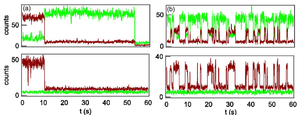
FIG. 3. Representative time traces of individual DNA molecules internally labeled with TMR and Cy5 fluorophores excited using alternating green and red lasers (0.5 and 0.13 kW/cm 2 , respectively). (a) TMR-6-Cy5 during green (top panel) and red excitations (bottom panel). (b) TMR-14-Cy5 during green (top panel) and red excitations (bottom panel). Note the perfect correlation between the acceptor emissions during green and red excitations.
