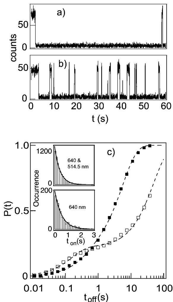
FIG. 4. The influence of green laser excitation on acceptor oscillations for the DNA-Cy5 construct. Typical time trace of the acceptor channel using (a) 640 nm and (b) 640+514 nm excitations. (c) Distributions of t_{\text{off}} and t_{\text{on}} for the DNA-Cy5 construct, excited by red (open symbols) or red+green lasers (filled symbols). A cumulative probability distribution P(t) is used to determine the on rates. P(t) is approximated by double-exponential fits (dotted lines), yielding on rates of 0.213 and 0.026 \text{s}^{-1} for the 640+514 nm excitation (filled symbols) and 640 nm excitation (open symbols), respectively. The insets are monoexponential distributions of the on times with the indicated excitation scheme yielding k_{\text{off}} \sim 2 \text{ s}^{-1} in both cases.
